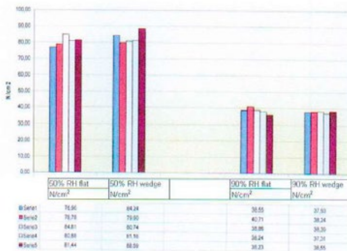
Load tests on load rests with 50% and 90% RH
